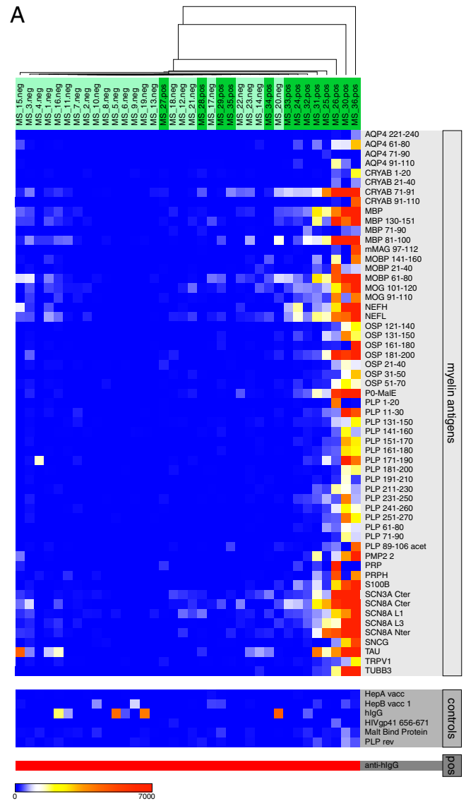
Fig. 2. IgG reactivity in B cell supernatants, comparing ELISpot-neg and ELISpot-pos samples. (A) Heatmap of antibody reactivity (in mean fluorescence intensity [MFI]) against 57 myelin antigens identified as significantly different between ELISpot-neg and ELISpot-pos B cell supernatants in SAM analysis ( Top ), nonmyelin controls ( Middle ), and positive control ( Bottom ). (B) Venn diagram indicating the number of overlapping significant antigens between the comparisons of ELISpot-neg vs. ELISpot-pos (supernatants) (orange) and HC/OND vs. ELISpot-pos (supernatants) (green). (C) Venn diagram indicating the number of overlapping significant antigens between the comparisons ELISpot-neg vs. ELISpot-pos (supernatants) (orange) and HC/OND vs. MS (plasma) (blue).
